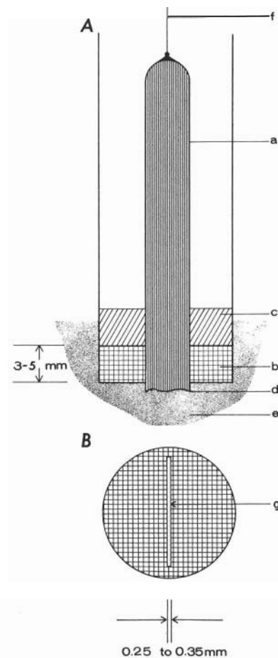
FIGURE 1. Diagram of the EMOC preparation. A, side view. B, bottom view. Only the cut end of the muscle is in direct contact with the labelled Ringer's solution. a, sartorius muscle; b, silicone rubber gasket; c, vaseline; d, cut end of muscle; e, bathing solution; f, anchoring string; g, slit in silicone rubber gasket. (From Ling, 1978. By permission of J. Physiol. )
