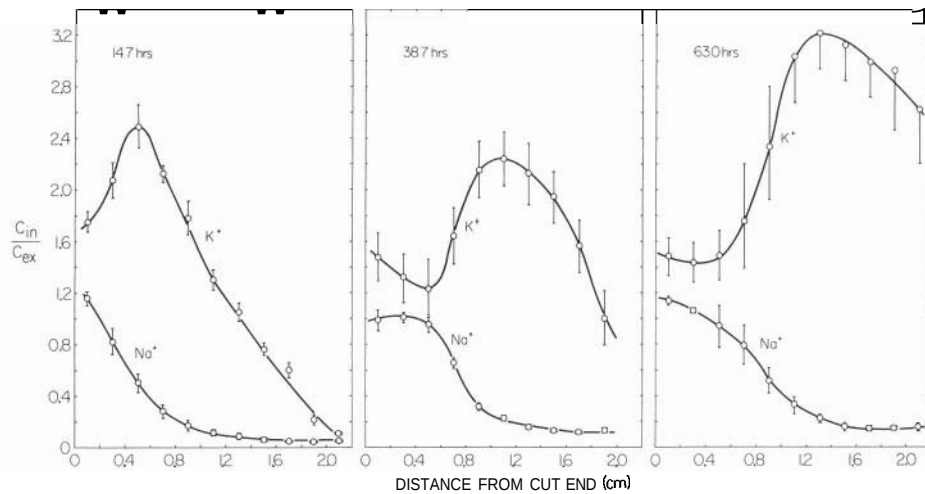
FIGURE 2. The simultaneous influx of labelled K^+ and labelled Na^+ into sartorius muscle through their cut ends. The three groups of frog sartorius EMOC preparations were exposed to normal Ringer's solutions labelled with both ^{42}K and ^{22}Na for 14.7, 38.7 and 63.0 hr, respectively. The abscissa represents the distance of the mid-point of each cut segment from the cut surface of the muscle fibers. The ordinate represents the ratio of the labelled ion concentrations in the water of each muscle segment ( C_{in} ) over the concentration of the same labelled ion in the solution bathing the cut end of the muscles at the conclusion of the experiment ( C_{ex} ). Each point was the average of 4 (14.7 hr), 10 (38.7 hr) and 4 (63.0 hr) experiments, respectively, the distance between the two longitudinal bars being twice the standard error. (From Ling, 1978. By permission of J. Physiol.)
