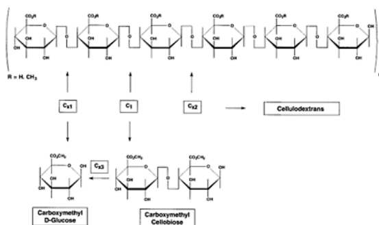
FIGURE 27.4 Diagrammatic representation of the action of cellulolytic enzymes on the substrate carboxymethyl cellulose (CMC). The \text{C}_1 enzyme (1,4- \beta -glucan cellobiohydrolase) hydrolyzes the 1–4 \beta bond on the nonreducing end of the polymer to yield carboxymethyl cellobiose molecules. \text{C}_{x3} or cellobiase (1,4- \beta -glucosidase) hydrolyzes cellobiose to yield carboxymethyl D-glucose residues, which is a reducing sugar. \text{C}_{x1} is exocellulase (1,4- \beta -exoglucanase) that cleaves one carboxymethyl D-glucose residue from the nonreducing end of the CMC molecule, whereas \text{C}_{x2} is an endocellulase (1,4- \beta -endoglucanase) that internally hydrolyzes bonds to produce various-length cellulodextrans. All of the cellulodextrans can be substrates for \text{C}_1 or \text{C}_{x1} enzymes, and thus \text{C}_{x2} may increase the apparent activity of the other enzymes by providing more substrate (if substrate is a limiting factor in the reaction mix). (Courtesy of Dr. J.Green, University of Tennessee.)
