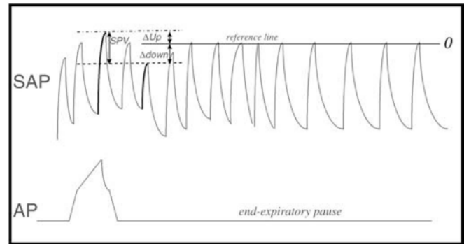
Fig. 2 Systolic pressure variation (SPV) after one mechanical breath followed by an end-expiratory pause. Reference line permits the measurement of \Delta_{up} and \Delta_{down} . Δup Maximal and minimal pulse pressure. AP Airway pressure; SAP systolic arterial pressure
