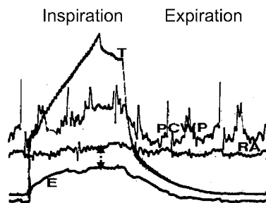
Fig. 1 Simultaneous recordings of tracheal pressure (T), pulmonary capillary wedge pressure (PCWP), right atrial pressure (RA), and esophageal pressure (E, as a surrogate for pleural pressure). During lung inflation (inspiration) pleural pressure increases more than right atrial (or central venous) pressure, leading to an inspiratory decrease in venous distending pressure (arrows)
