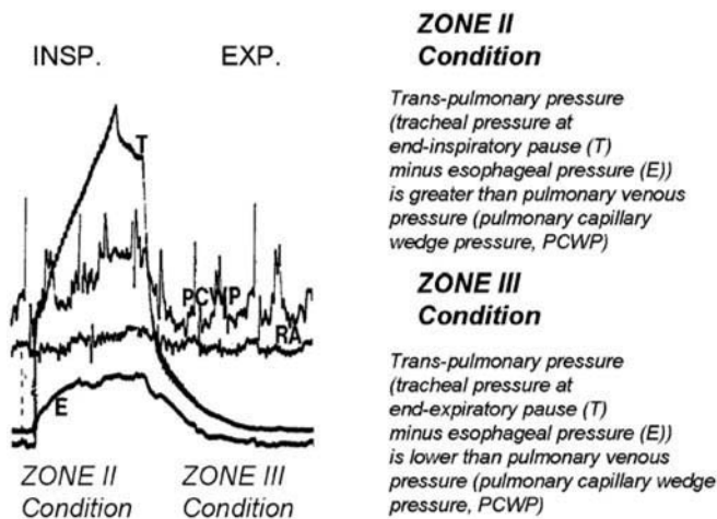
Fig. 2 An example of simultaneous recording of esophageal pressure (E), reflecting pleural pressure, right atrial pressure (RA), pulmonary capillary wedge pressure (PCWP), reflecting pulmonary venous pressure, and tracheal pressure (T). During the period of no-flow (end-inspiratory pause and end-expiration), T reflects alveolar pressure. Whereas a zone 3 condition is observed at end-expiration (PCWP > T), a zone 2 condition is realized at end-inspiration (T > PCWP). Also note that the increase in E during mechanical inspiration is accompanied by a similar increase in PCWP
