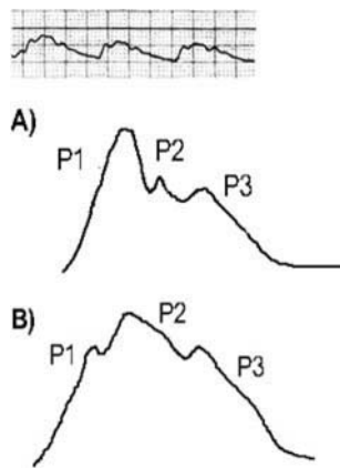
Fig. 1 The intra-cranial pressure waveforms. The upper tracing is an example of an ICP waveform from a patient monitoring system in which can be identified the three distinct components, as indicated in the text. A depicts the situation of a compliant system, B A high pressure wave recorded from a non-compliant system in which P2 exceeds the level of the P1 waveform, due to a marked decrease in cerebral compliance
