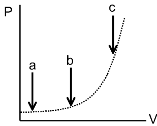
Fig. 2 Pressure-volume curve of the craniospinal compartment. This figure illustrates the principle that in the physiological range, i.e. near the origin of the x-axis on the graph (point a ), intracranial pressure remains normal in spite of small additions of volume until a point of decompensation (point b ), after which each subsequent increment in total volume results in an ever larger increment in intracranial pressure (point c )
