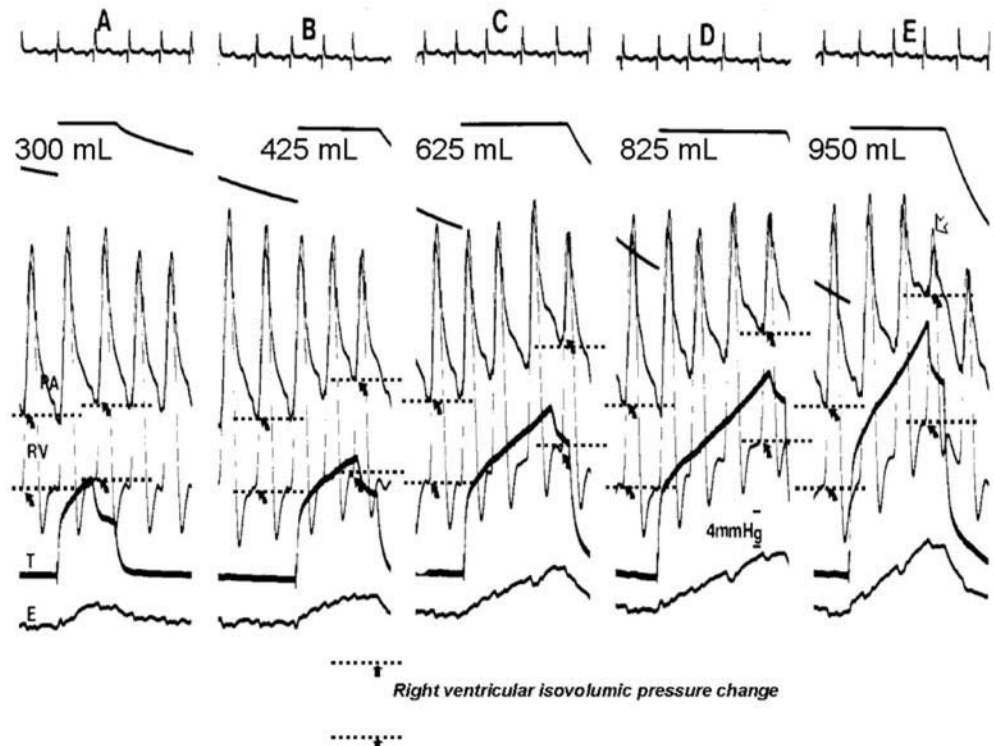
Fig. 3 Simultaneous recordings of expiratory volume (EV, ml), pulmonary artery pressure (PA, mmHg), right ventricular pressure (RV, mmHg), tracheal pressure (T, mmHg) and esophageal pressure (E, mmHg), during a progressive increase in tidal volume from 300 to 950 ml. This progressive increase in tidal ventilation required a progressive increase in the pressure developed by the RV during its isovolumetric contraction to open the pulmonary valve (i.e., the difference between pulmonary artery diastolic pressure, small closed arrow , and right ventricular end-diastolic pressure, small closed arrow ). Note also that, with the highest tidal volume ( right panel, E ), pulmonary artery pulse became negligible ( small open arrow )
