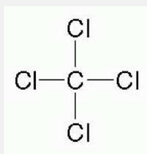
Figure 3-1. The carbon tetrachloride molecule.
