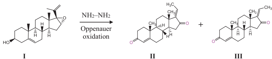
Scheme 1 Synthesis of stereoisomers of guggulsterone from 16,17-epoxypregnenolone ( I ) refluxed with hydrazine hydrate
