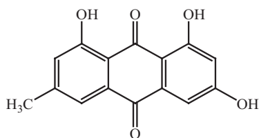
Emodin
