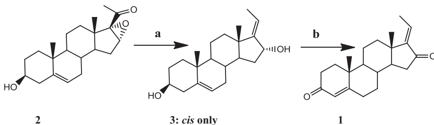
Scheme 4 Regioselective synthesis of E -guggulsterone from 16,17-epoxypregnenolone ( 2 ) and conversion of E -guggulsterone into the corresponding Z -isomer. (a) KOH, \text{NH}_2\text{NH}_2 monohydrate, di(ethylene glycol), 160^\circ\text{C} for 2 h (91% yield); (b) \text{Al}(\text{O}-i\text{-propyl})_3 , cyclohexanone, benzene, 80^\circ\text{C} for 2 h (92% yield)
