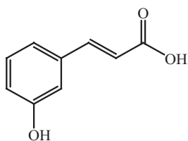
m-coumaric acid
