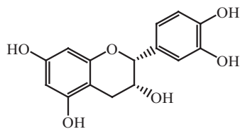
Epicatechin
