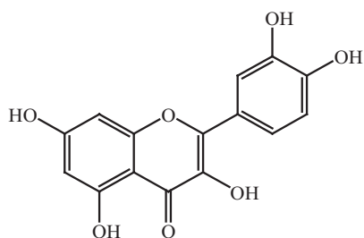
Quercetin
